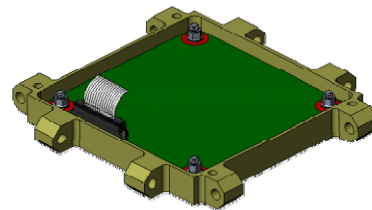
Figure 4. A nanomodule (Cubesat component), based on the 1 \times 1 nanomodular format (NMF), which doubles as a panel for the Cubesat.
