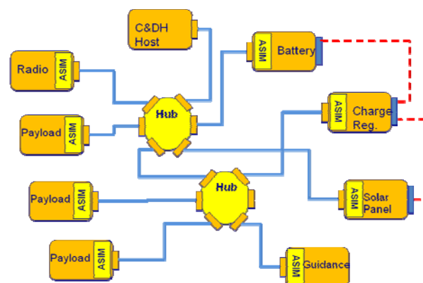
Figure 10. SPA-U network (solid interfaces are SPA-U connections; dashed interfaces are specialty power generation bus connections).
