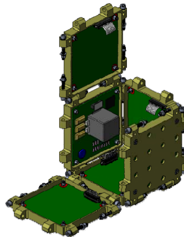
Figure 5. View of CubeSat base on arrangement of six 1 \times 1 nanomodular format (NMF) nanomodules, in opened view. Nanomodules are mounted within the panels and the structure is folded up into a cube.
